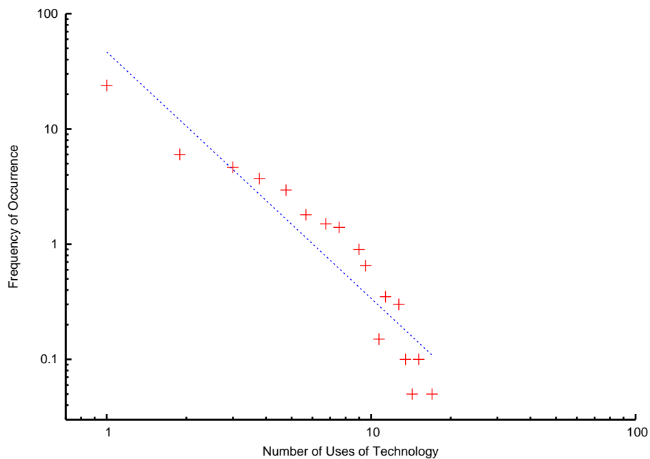
Figure 7: Very few key technologies are used heavily to directly construct new ones. The plot shows the average over 20 experiments at their termination of 250,000 steps each.
