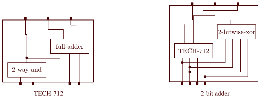
Figure 2: TECH-712 is useful towards satisfying the 2-bit-adder goal since the two high-order bits are computed correctly. (The low-order bit is on the left. For multi-bit adders, input bits are interleaved.)
