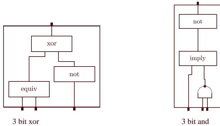
Figure 1: two circuits “invented” for simple goals.
