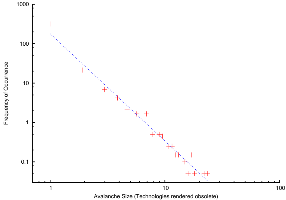
Figure 8: Gales of destruction (or avalanches of collapse in use), average over 20 experiments.
